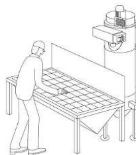
磨砂作业 Polishing
